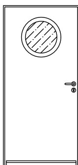
Hermes V U_d=1.2 (HB) U_d=1.5 (HM)
